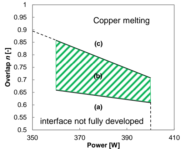
Figure 5 - Process window for homogenous interface
