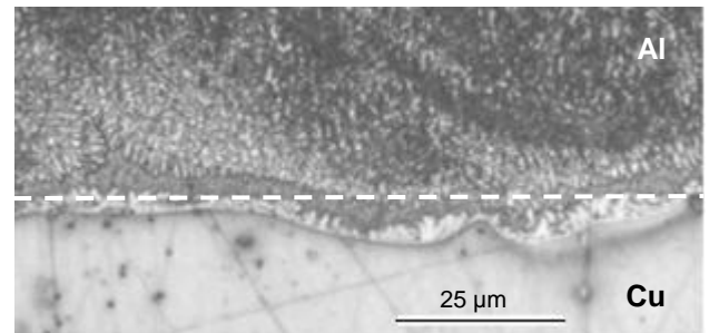
Figure 6 - Wavy interface in longitudinal section
