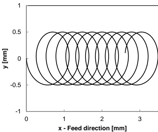
Figure 3 - Superposed circular beam movement
