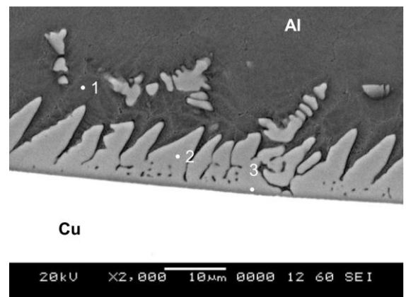
Figure 7 - SEM image of the interface
